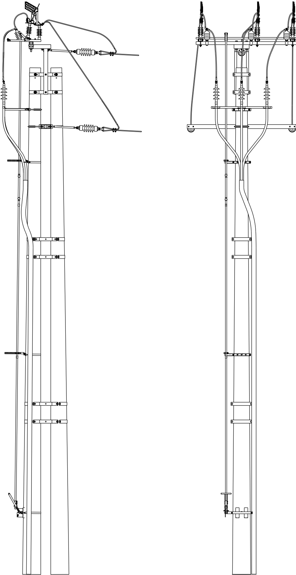
Switch disconnector with earthing type SRUN-24 with OPSPE kit on a OP11 pillar with cable head
